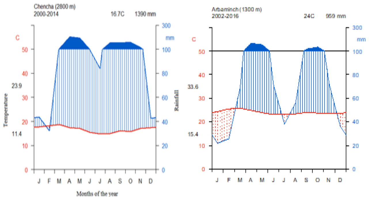
Figure 3. Walter's and LiethClima diagram of Chencha and Arba Minch stations.
